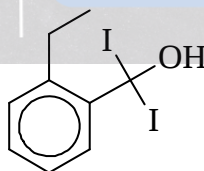
compound X
