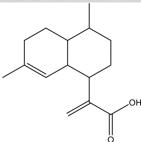
artemisinic acid
