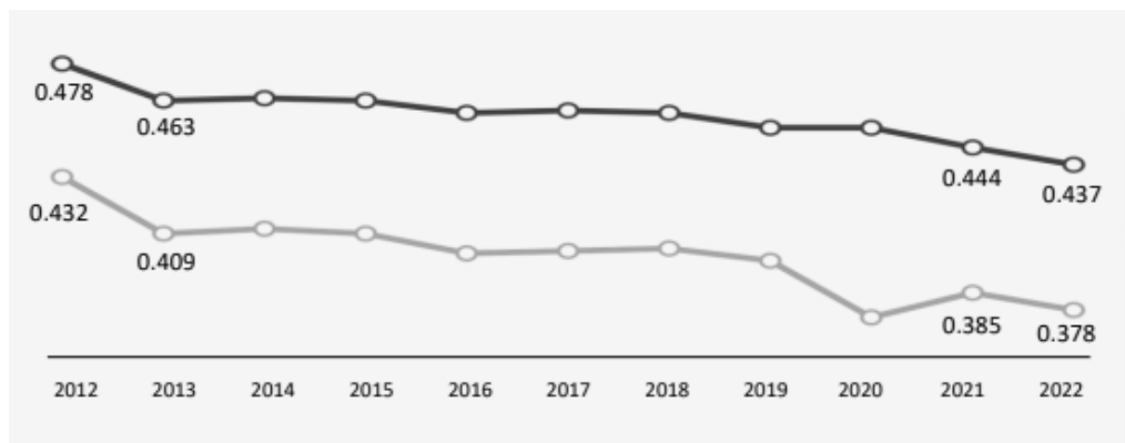
Figure 3: Gini Coefficient in Singapore
