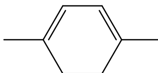
1,4-dimethylcyclohexa-1,3-diene
