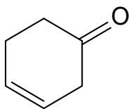
cyclohex-3-en-1-one
