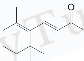
\beta -ionone
